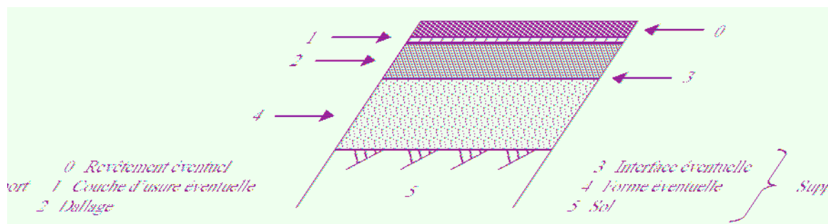
Figure 11 Constitution d'un dallage (Source DTU 13.3)
